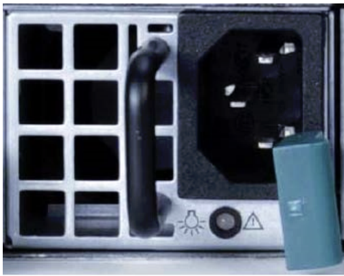
Figure 18. Removing a PSU from the chassis
